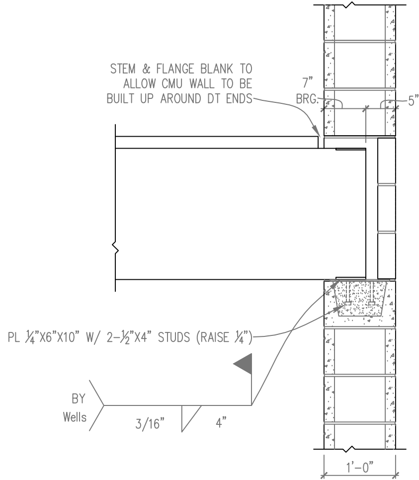
DT PANEL BEARING ON CMU BLOCK - AT MEZZ. DETAIL SCALE: \frac{3}{4} " = 1'-0"
