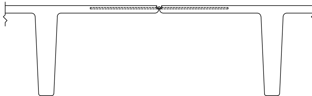
A DT ROOF TYPICAL WELD POINT DETAIL SCALE: 3/4" = 1'-0"
