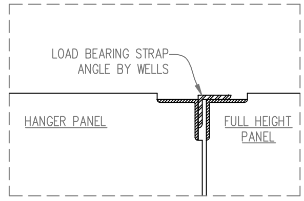
A HANGER BEARING CONDITION DETAIL SCALE: 1" = 1'-0"
