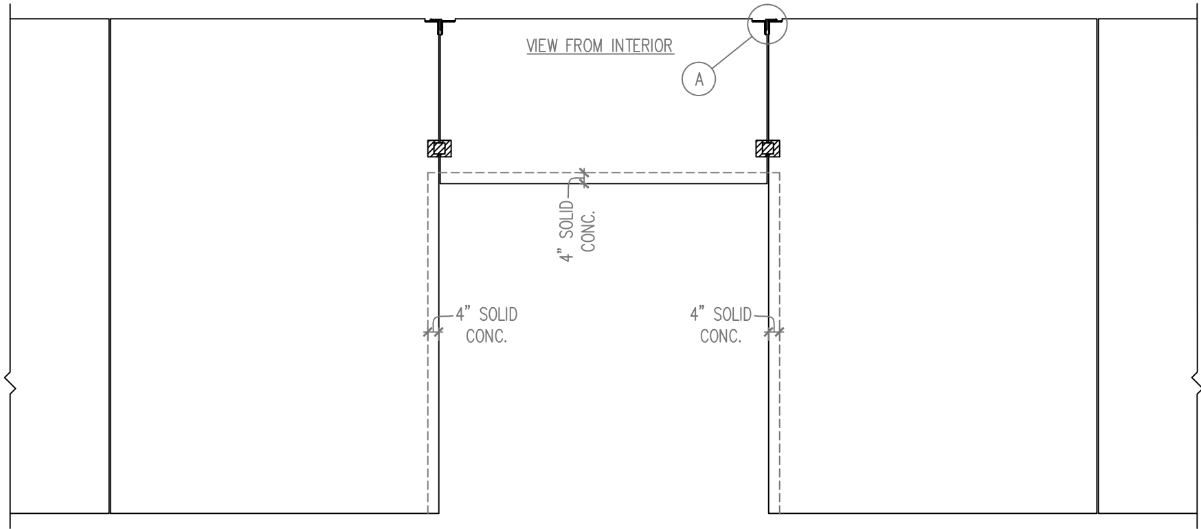
- OVERHEAD PANEL – NON LOAD BEARING HANGER DETAIL SCALE: 1/4" = 1'-0"
