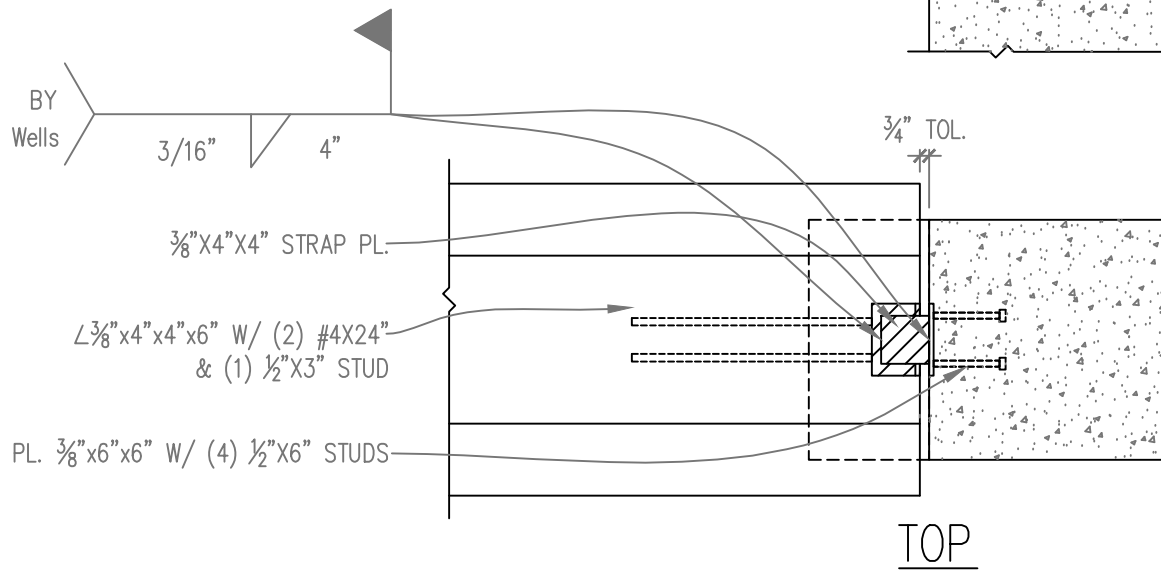
- INVERTED TEE BEAM BEARING ON COLUMN HAUNCH DETAIL SCALE: \frac{3}{4} " = 1'-0"
