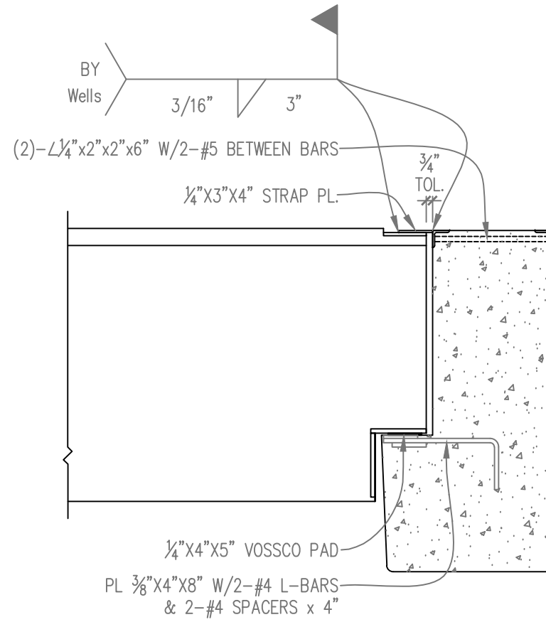
- COPED DT BEARING ON L BEAM DETAIL SCALE: 3/4" = 1'-0"
