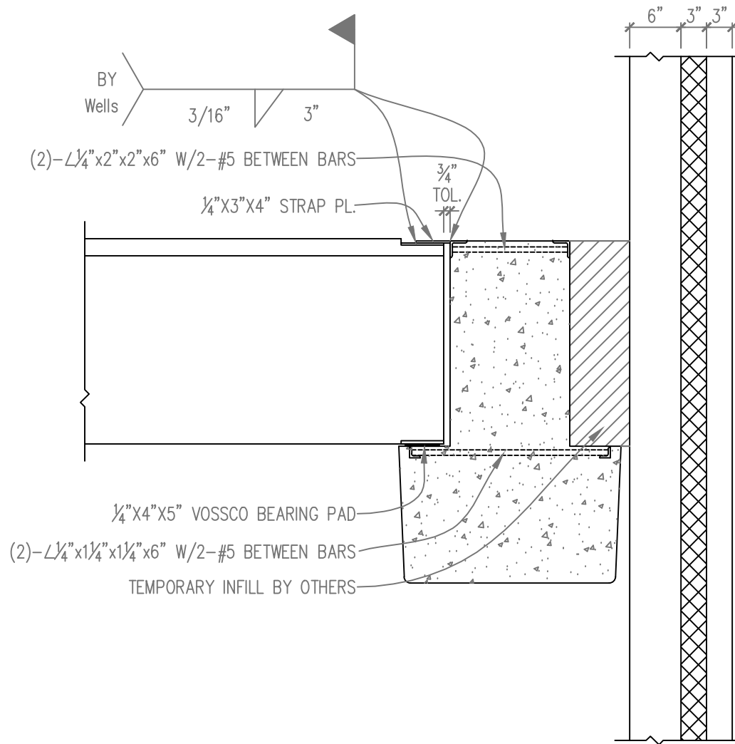
DT BEARING ON INVERTED TEE BEAM - FUTURE EXPANSION SCALE: 3/4" = 1'-0"
