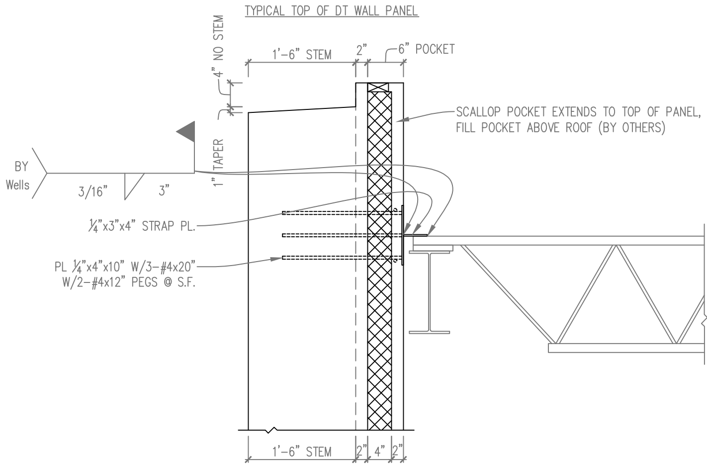
DT WALL TO STEEL JOIST ON BEAM SCALE: 3/4" = 1'-0"
