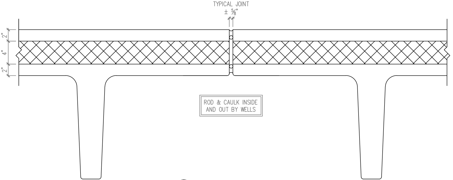
— TYPICAL CAULK JOINT DETAIL SCALE: 1 1/2" = 1'-0"
