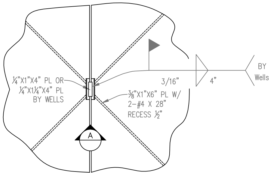
- DT WALL - WELD POINT DETAIL SCALE: 3/4" = 1'-0"
