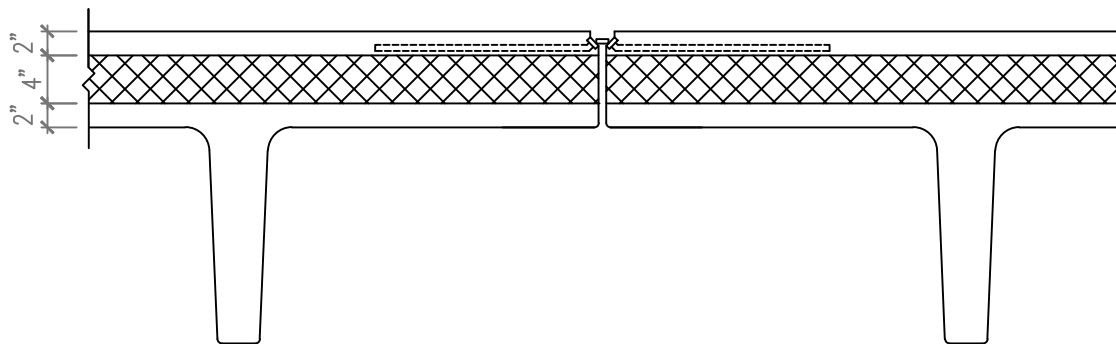
A DT WALL - WELD POINT DETAIL SCALE: 3/4" = 1'-0"
