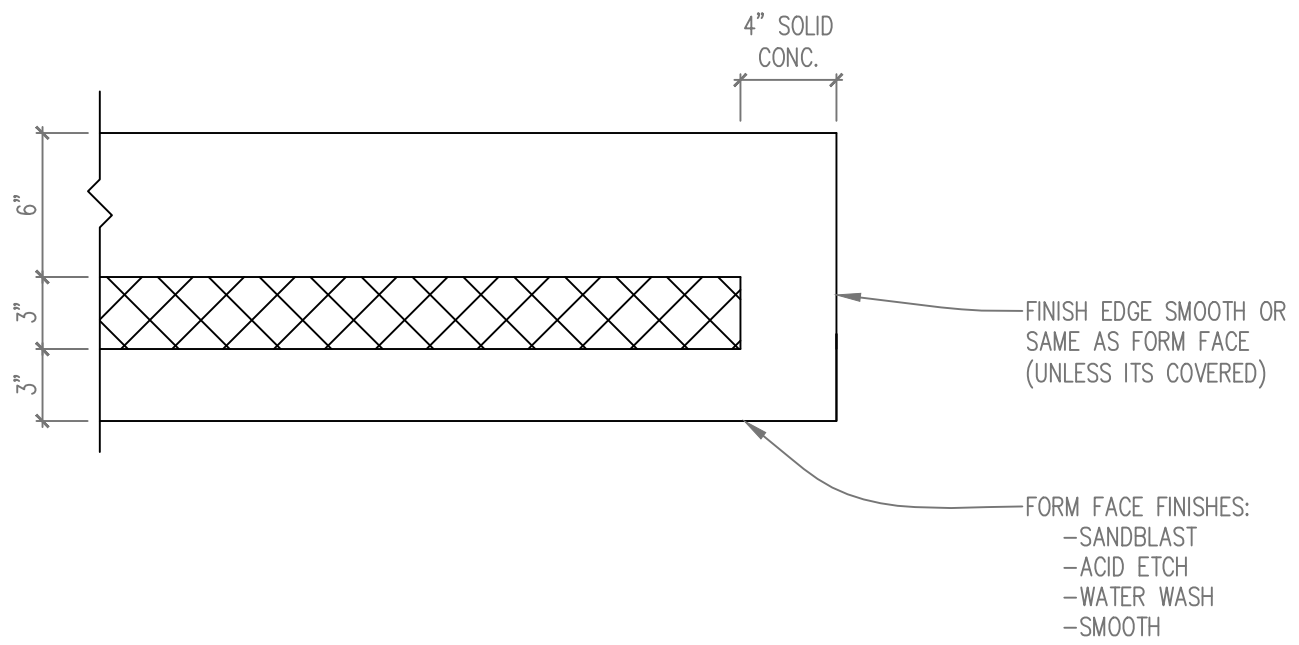
- FINISHES @ OPNG - SOLID CONC. DETAIL SCALE: 1 1/2" = 1'-0"
