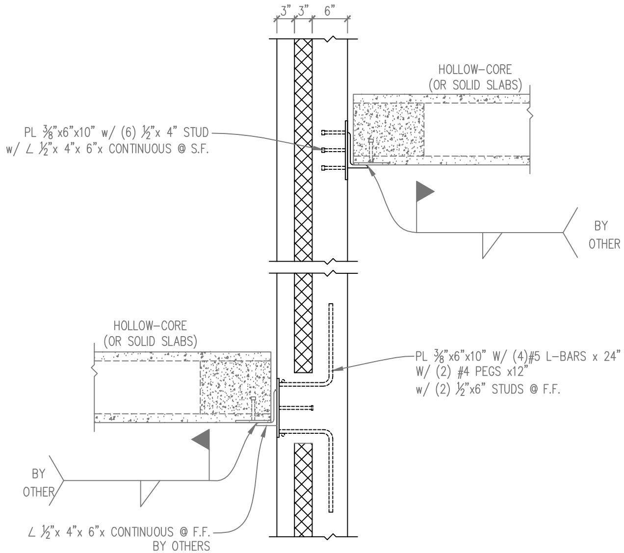
— PLANK BEARING DETAIL (DETAIL) SCALE: \frac{3}{4} " = 1'-0"
