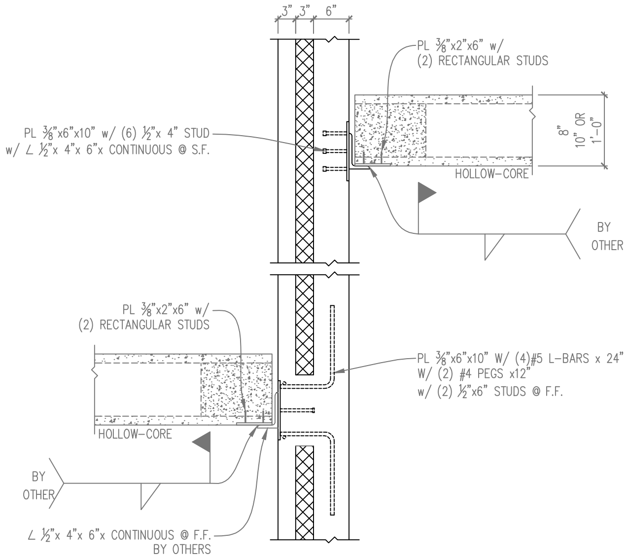
— HOLLOW-CORE BEARING ON PRECAST WALL DETAIL SCALE: \frac{3}{4} " = 1'-0"
