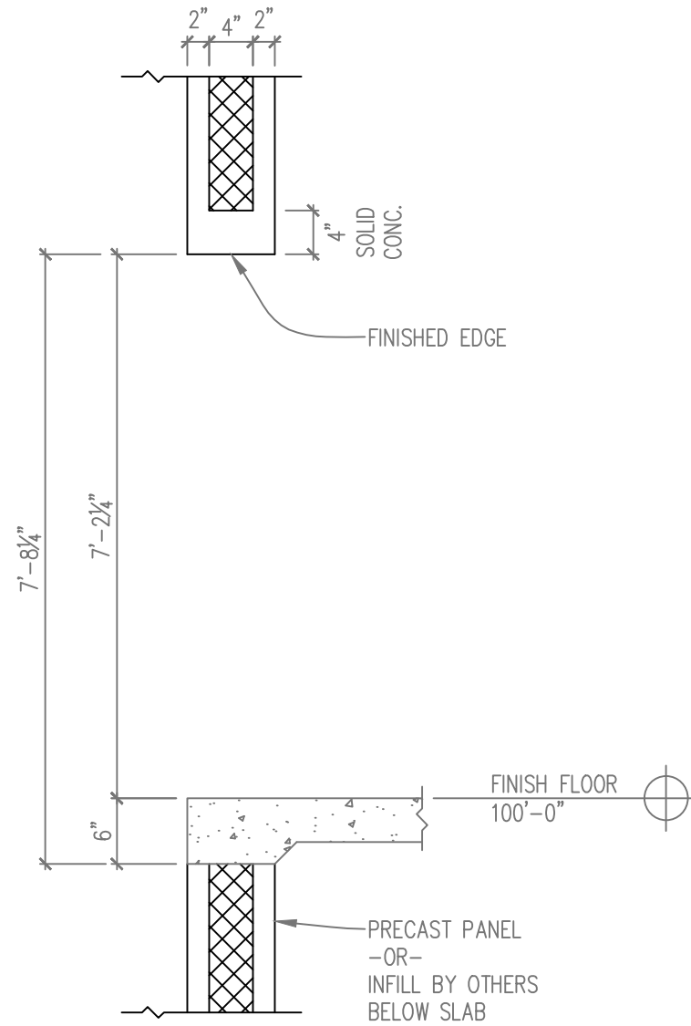
OPNG DETAIL - SOLID CONC. AT HEAD SCALE: 3/4" = 1'-0"
