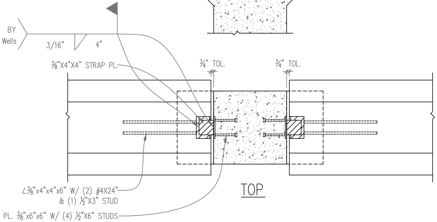
- TWO INVERTED TEE BEAMS BEARING ON COLUMN HAUNCHES DETAIL SCALE: 3/4" = 1'-0"
