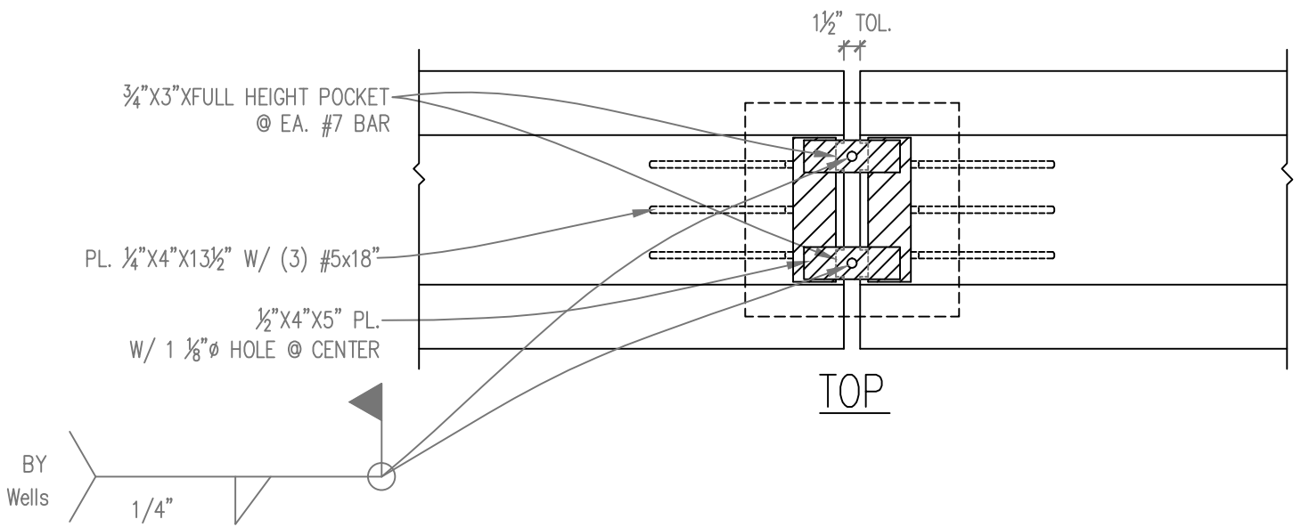
— INVERTED TEE BEAMS SPLIT BEARING ON COLUMN (DETAIL) SCALE: 3/4" = 1'-0"
