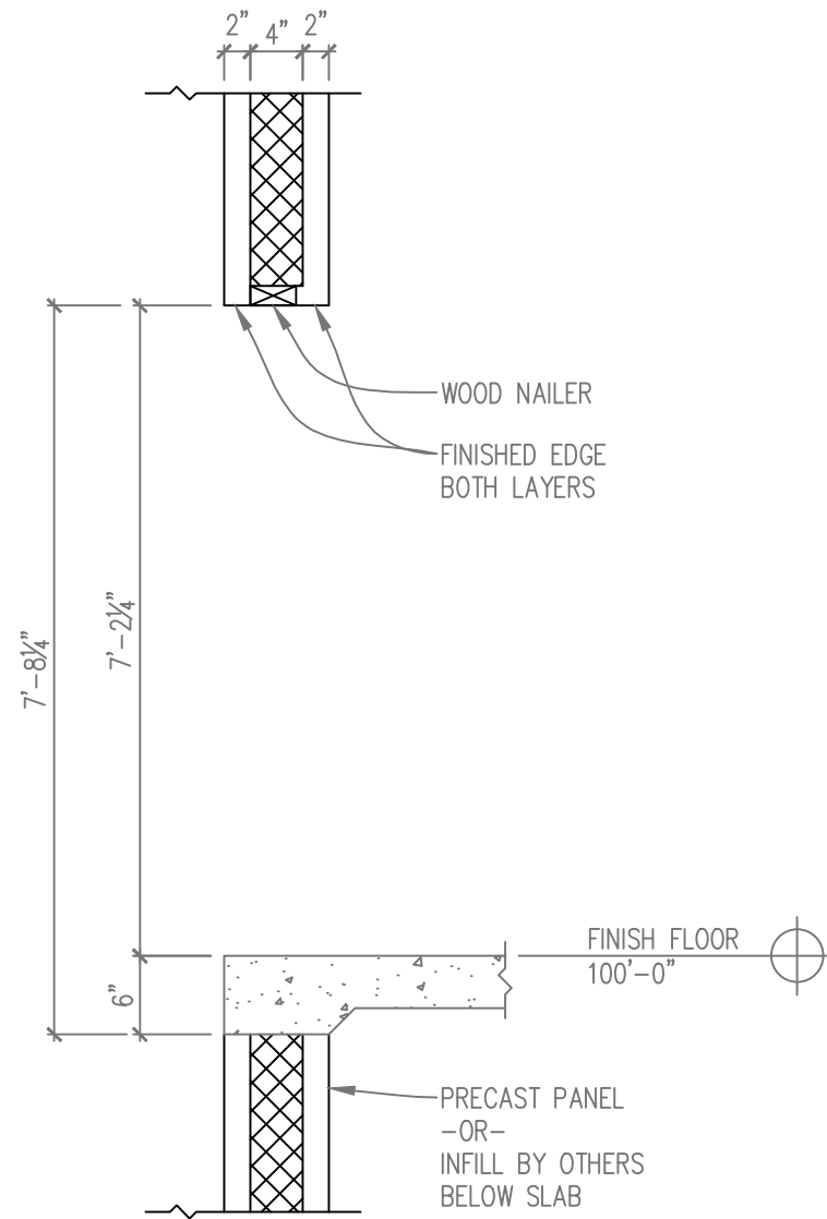
OPNG DETAIL - WOOD NAILER AT HEAD SCALE: 3/4" = 1'-0"
